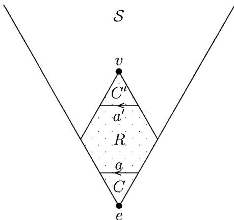
FIG. 6. Convex hull R of C and v .
