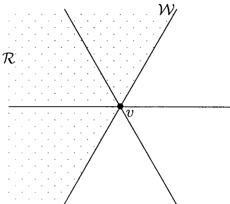
FIG. 2. A root \mathcal{R} containing the vertex v .
