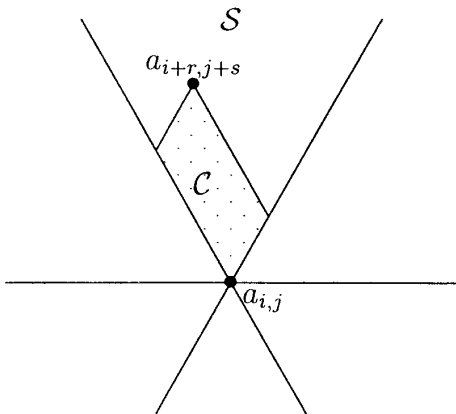
FIG. 10. Convex hull \mathcal{C} of a_{i,j} and a_{i+r,j+s} .
