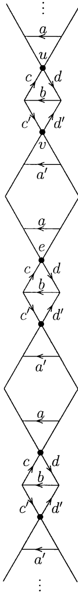
FIG. 8. Infinite tessellation of the region R' .
