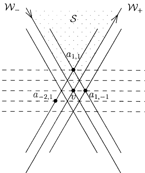
FIG. 5. Labelling of an apartment with respect to a sector \mathcal{S} .
