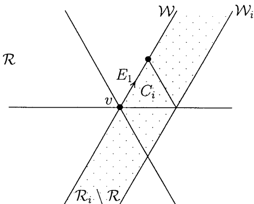
FIG. 3. Extending the root \mathcal{R} to a root \mathcal{R}_i .
