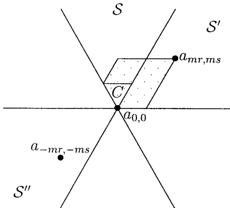
FIG. 9. Illustration of the proof of case 3 with r > 0 and s < 0 .
