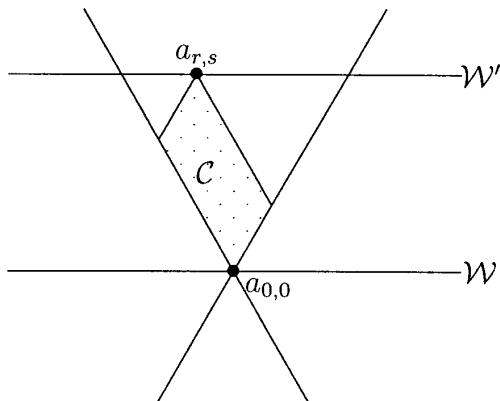
FIG. 11. Strip between walls \mathcal{W} and \mathcal{W}' showing convex hull \mathcal{C} of a_{0,0} and a_{r,s} .
