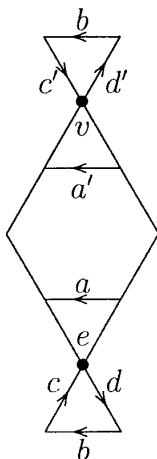
FIG. 7. The region R' .
