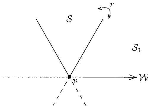
FIG. 13. Implementation of correspondence in \mathcal{A} .
