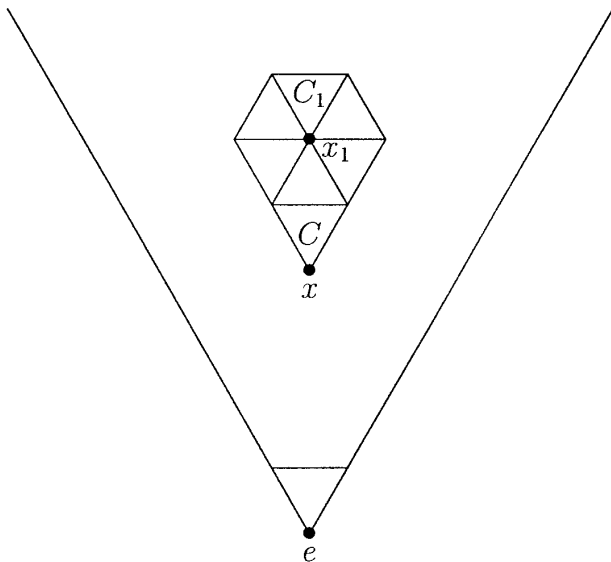
FIG. 16. Relative positions of x, x_1, C, and C_1 .
