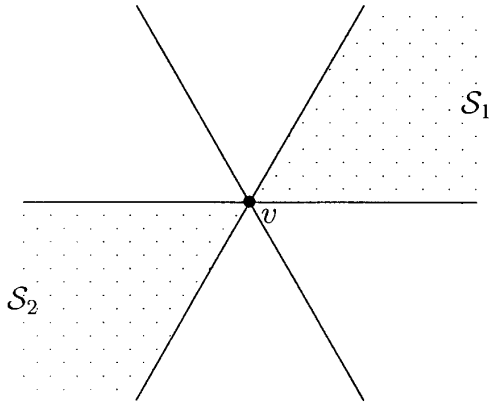
FIG. 1. Opposite sectors in an apartment.
