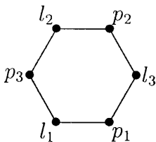
FIG. 15. Incidence diagram for point line pairs \{p_2, l_2\} corresponding to chambers D .
