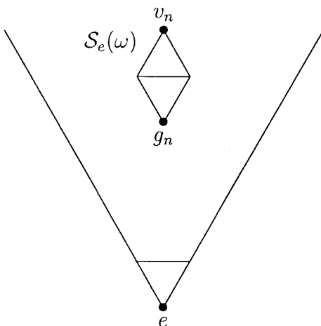
FIG. 14. Relative positions of v_n and g_n .
