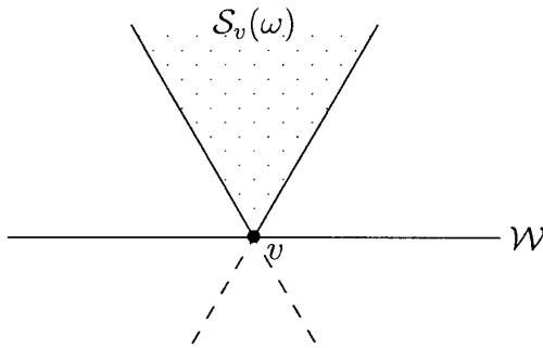
FIG. 12. Geometric interpretation of second case.
